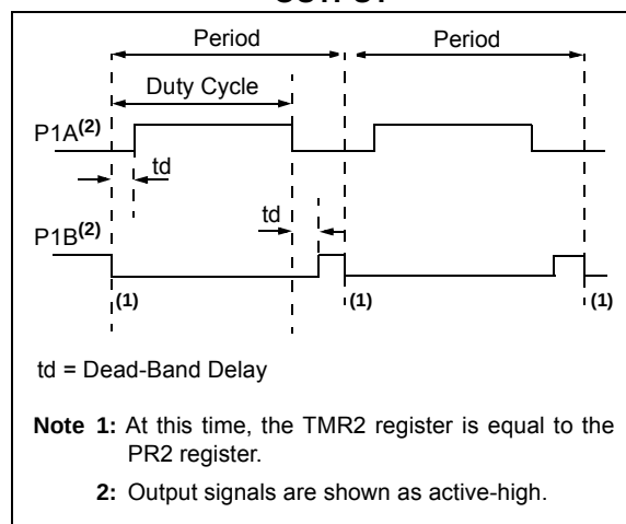
FIGURE 16-4: HALF-BRIDGE PWM OUTPUT
