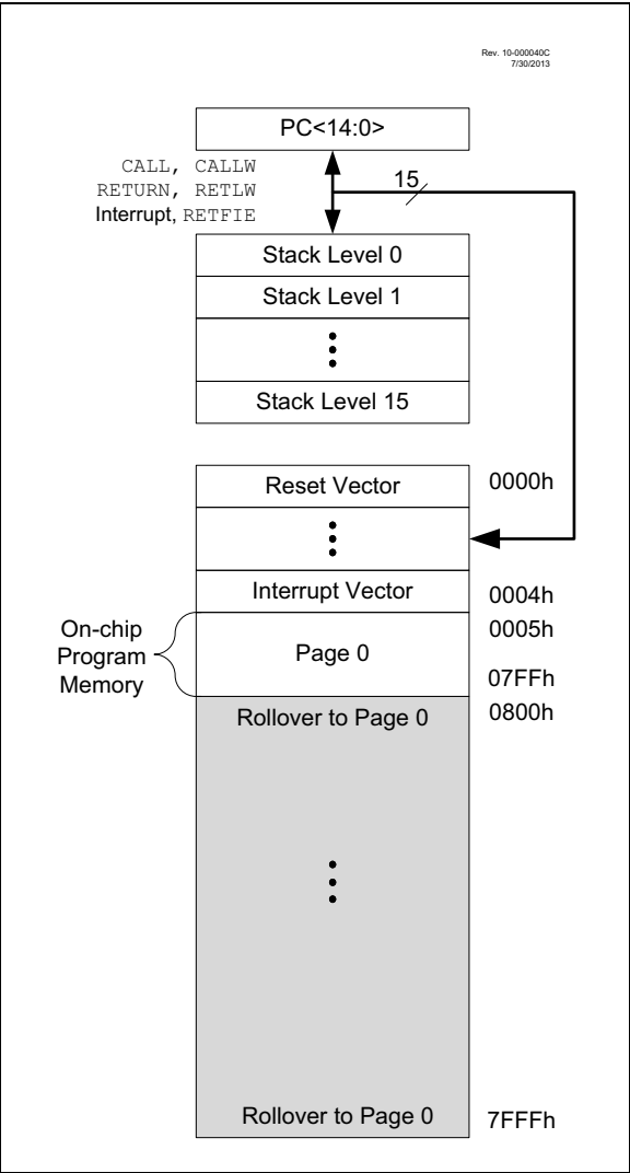
FIGURE 3-1: PROGRAM MEMORY MAP AND STACK FOR PIC16(L)F1503
