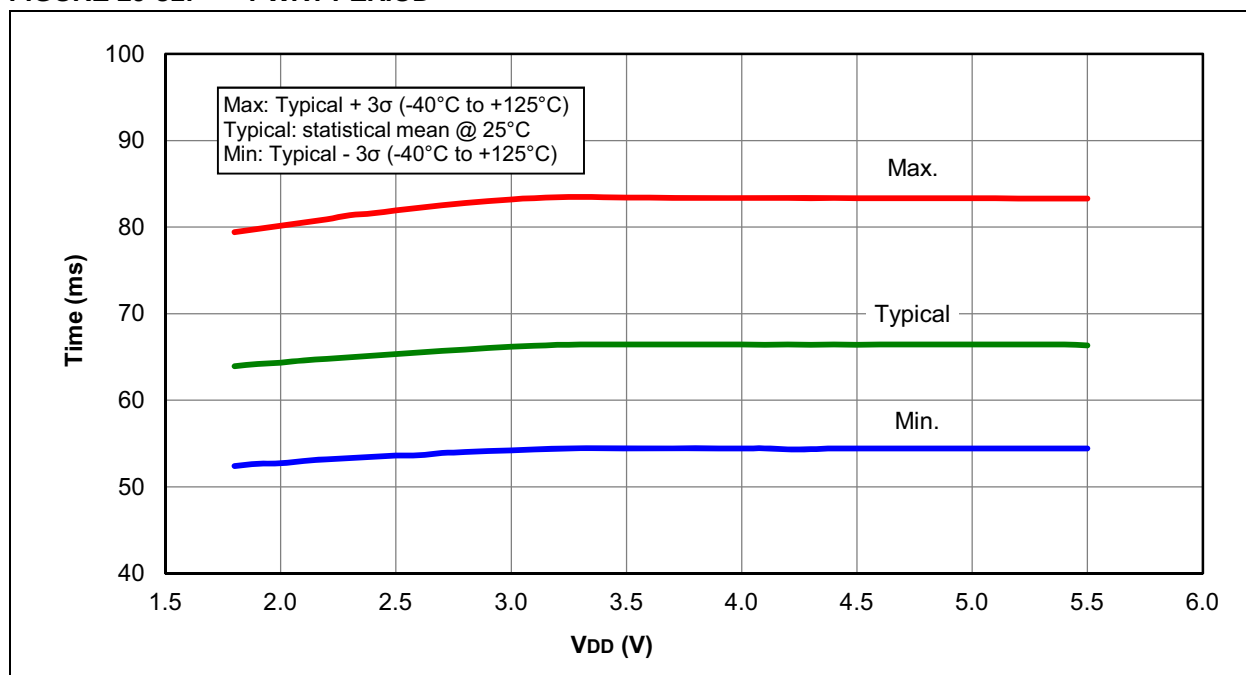
FIGURE 29-51: PWRT PERIOD
